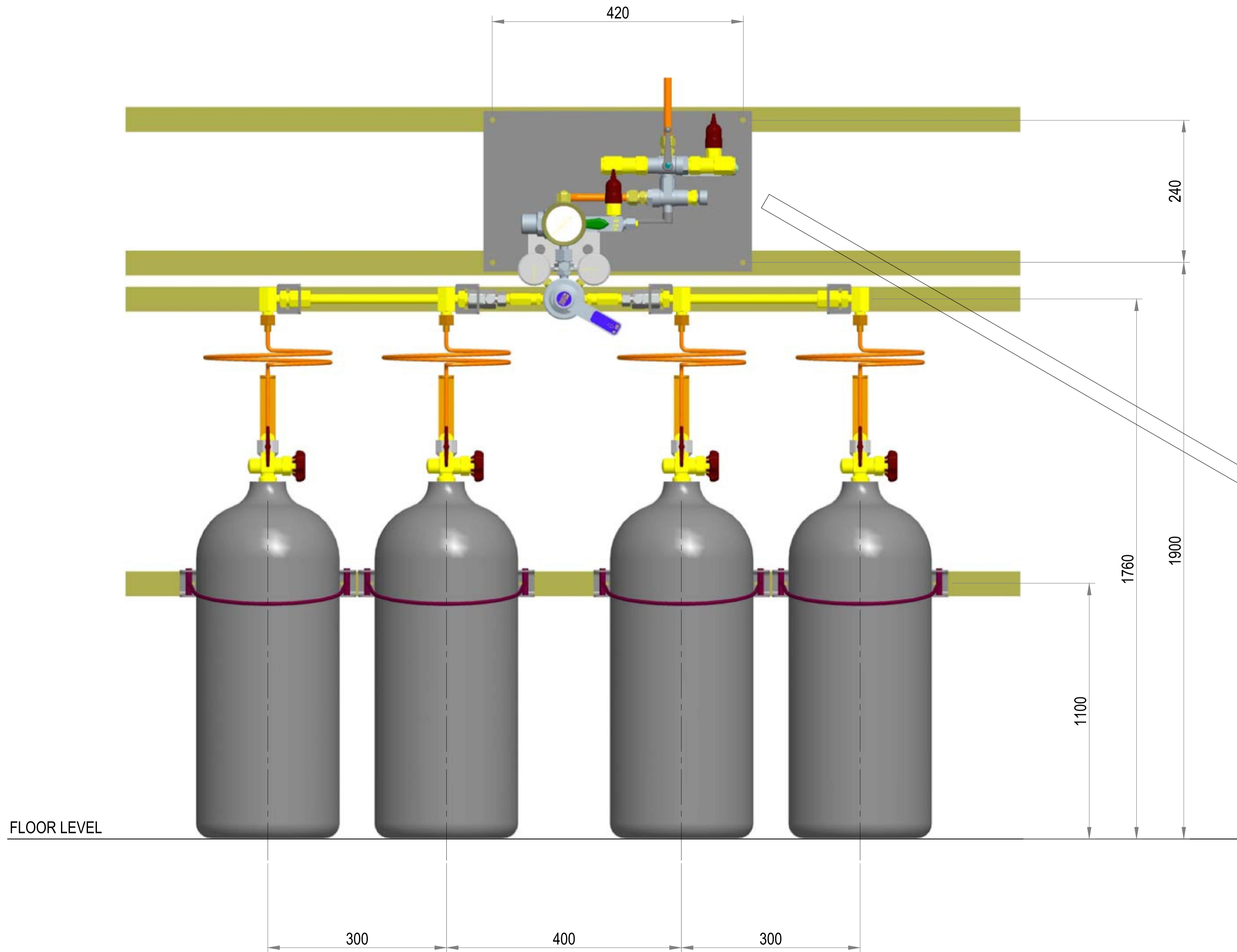
AUTO CHANGE-OVER MANIFOLD WITH CYLINDER BANK NOT TO SCALE
